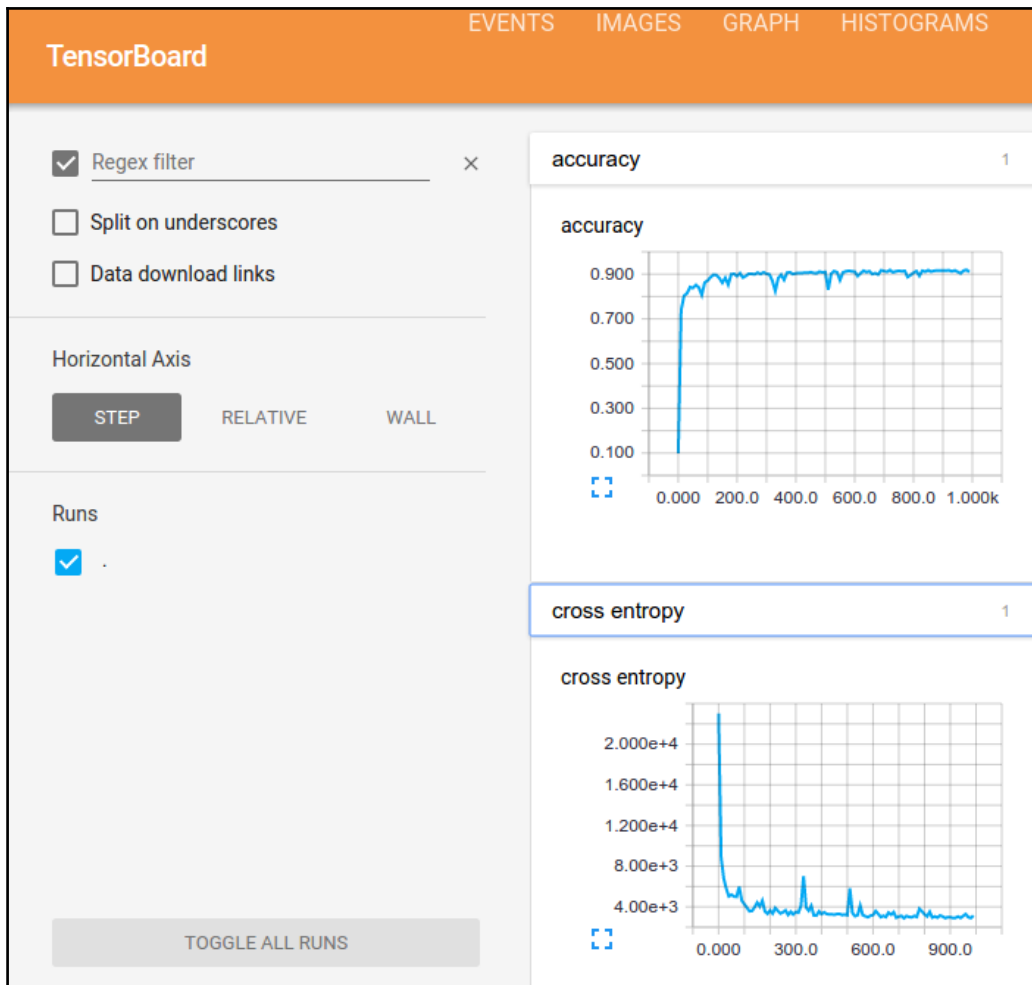
TensorBoard GUI
