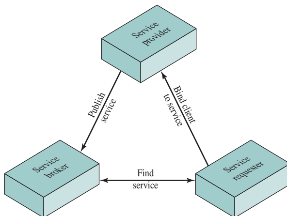
Figure 16.10 SOA Model
