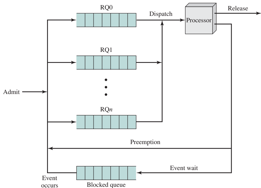
Figure 9.4 Priority Queueing
