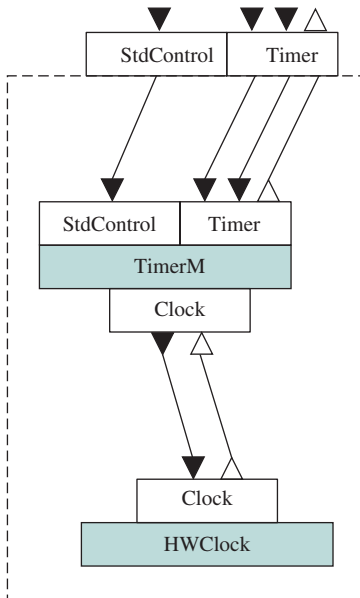
(b) TimerC configuration
