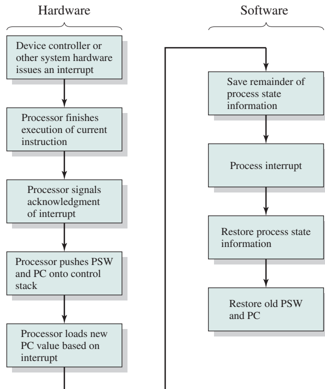
Figure 1.10 Simple Interrupt Processing
