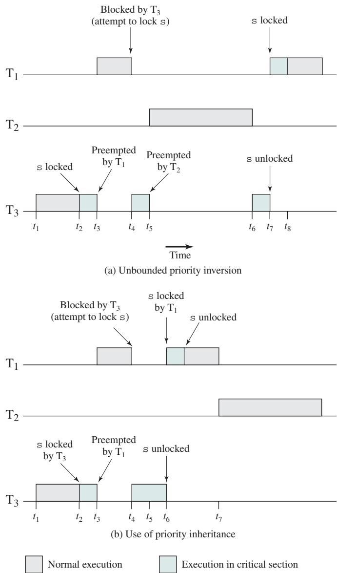
Figure 10.9 Priority Inversion
