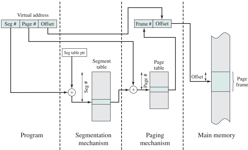
Figure 8.13 Address Translation in a Segmentation/Paging System
