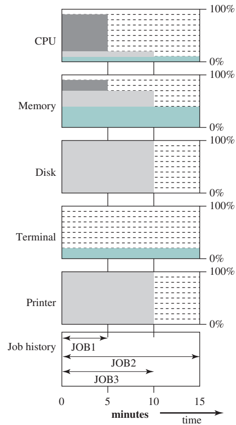
(b) Multiprogramming
